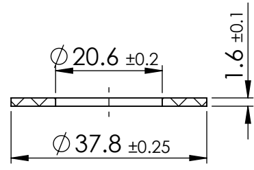
SECTION X-X
